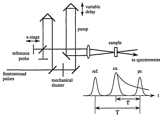
Fig. 1. Experimental setup of the frequency-domain interferometer and the time sequence of the pump (ex.), probe (pr.), and reference (ref.) pulses with separation \tau and T .
